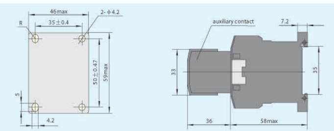
Dimensions: 3 & 4 Pole Contactor
