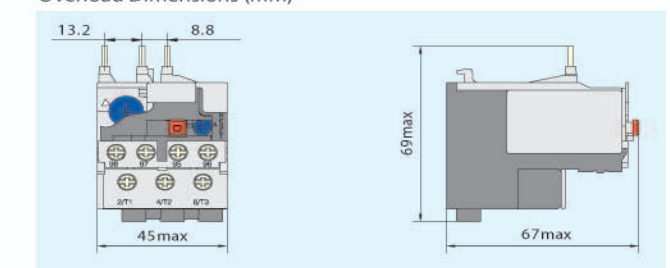
Overload Dimensions (mm)
