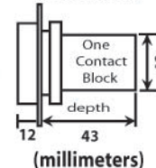
Pushbutton Dimensions
